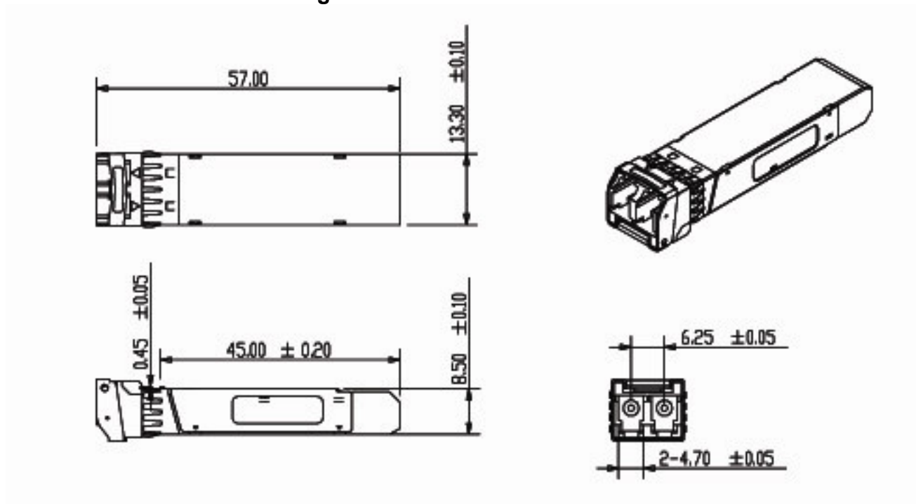
Figure3. Host-Module Interface
